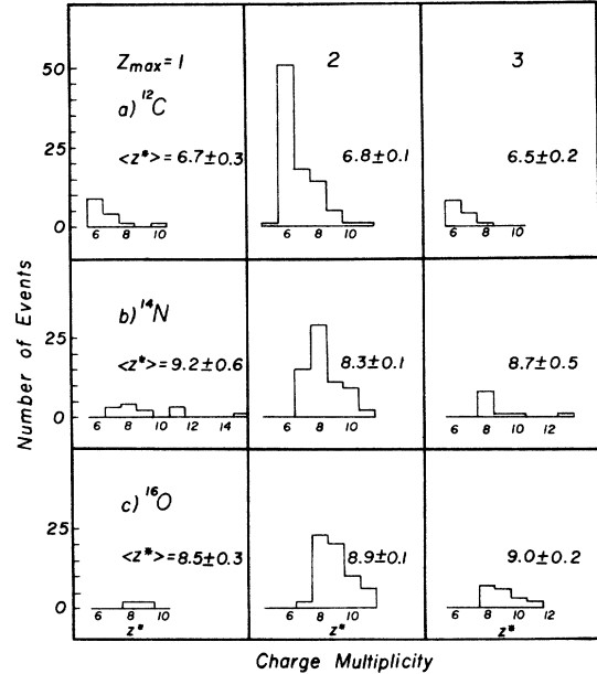
FIG. 8. Histograms of the charge multiplicity distributions for the fragmentation of (a) ^{12}\text{C} , (b) ^{14}\text{N} , and (c) ^{16}\text{O} . The quantity Z^* = \sum_{i=1}^n |Z_i| , where |Z_i| is the absolute charge of the n th prong. The histograms are based upon the same events used for Fig. 7, and are also ordered as to Z_{\max} . The mean-charge multiplicity is indicated for each distribution.
