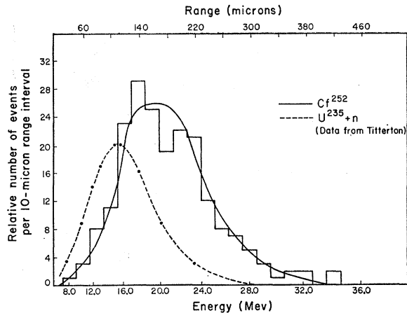
FIG. 2. Energy spectrum of long-range alpha particles associated with fission. Solid curve, \text{Cf}^{252} ; dashed curve, \text{U}^{235}+n (data from Titterton 26 ).
