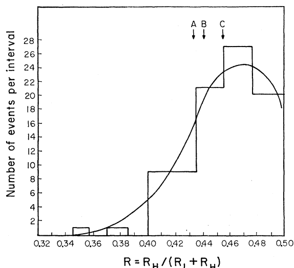
FIG. 5. Number of events vs R for fission fragments associated with long-range alpha-particle emission in fission of U 235 induced by thermal neutrons. (A) Mean value of R for ordinary fission from J. K. Bøggild, K. H. Brostrom, and T. Lauritsen, Kgl. Danske Videnskab. Selskab, Mat.-fys. Medd. 18, No. 4, 1 (1940). (B) Mean value of R for ordinary fission from P. Demers, Phys. Rev. 70, 974 (1946). (C) Mean value of R for fission accompanied by alpha emission.
