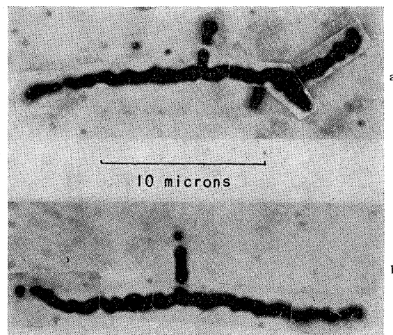
FIG. 7. Example of fission of Cf 252 with emission of light charged particle of short range.
