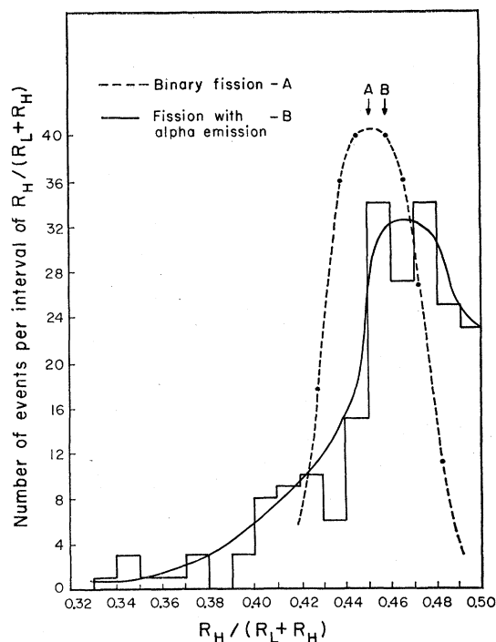
FIG. 6. Number of events vs R for fission fragments associated with long-range alpha-particle emission in Cf 252 . Dashed curve, binary fission of Cf 252 ; A denotes mean value of R . Solid curve, fission accompanied by alpha emission; B denotes mean value of R .
