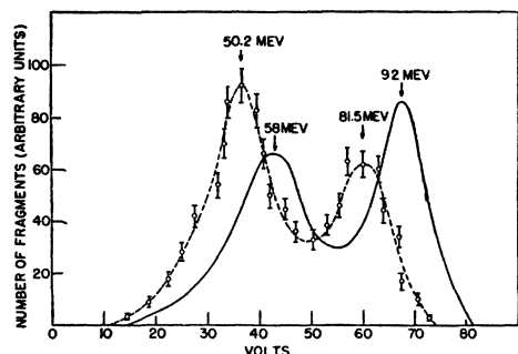
FIG. 12. Energy distribution of fission fragments. Solid curve is the normal distribution. Broken curve is the distribution in energy of fragments in coincidence with long-range \alpha -particles.
