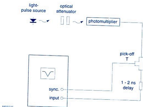
Fig.4.6 Set-up for measuring pulse response
