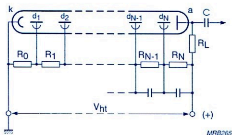
Fig.5.1 Positive-polarity voltage supply
