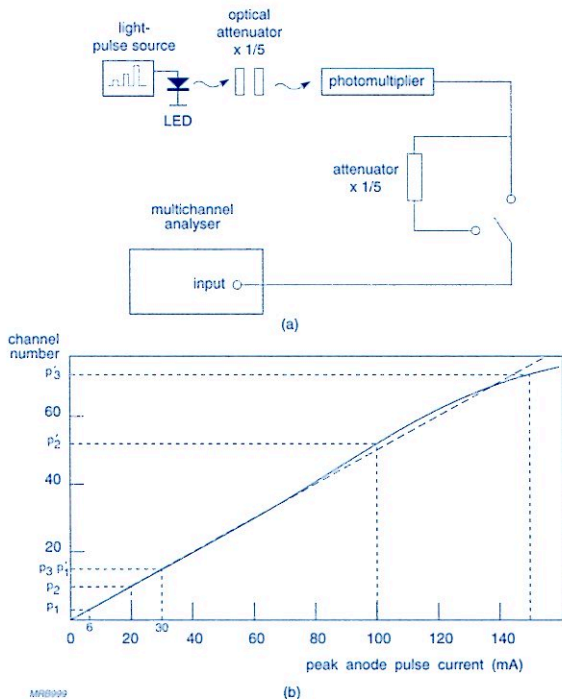
Fig.4.19 Pulse-linearity test; (a) block diagram of the 'three-pulses method'; (b) example of an experimental linearity curve obtained with the three-pulses method (channel number in arbitrary units)
