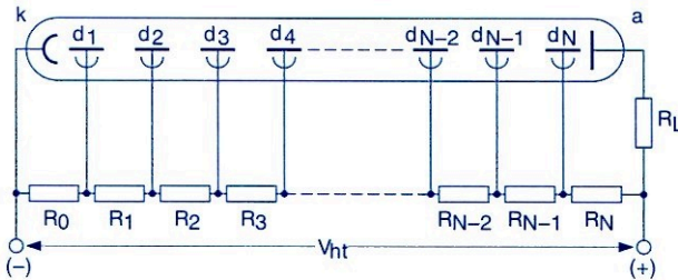
Fig.1.2 Voltage-divider high-tension supply
