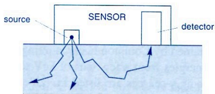
Fig.7.13 Soil density measurement by means of Compton scattering
