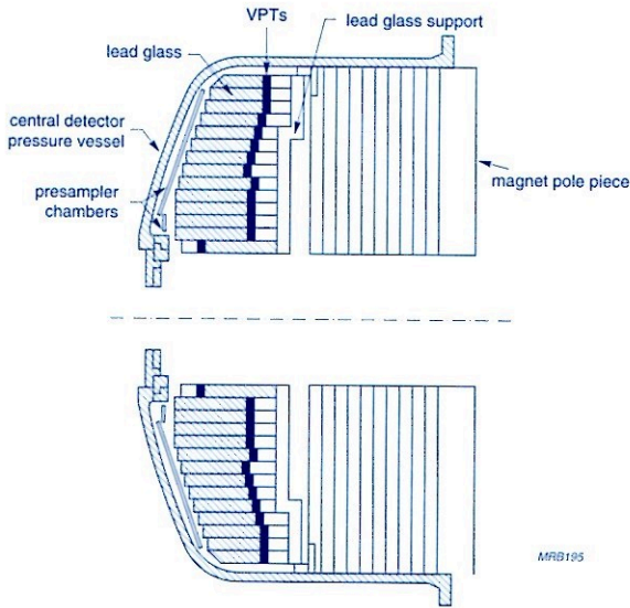
Fig.7.16 Lead-glass calorimeter end caps and Photonis VPTs (courtesy of OPAL collaboration, CERN, Geneva)
