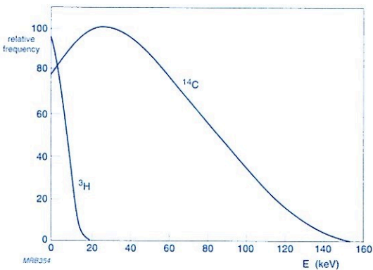
Fig.7.5 Relative spectral energy E of \beta emission from tritium ( ^3\text{H} ) and carbon ( ^{14}\text{C} )
