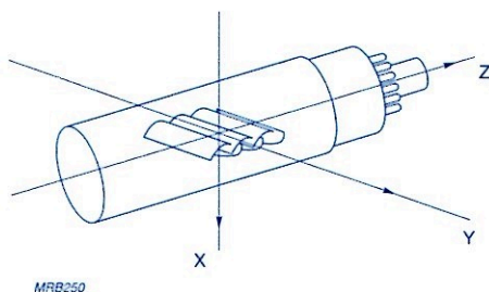
Fig.4.35 Axes used in measuring magnetic sensitivity
