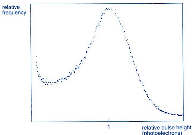
Fig.2.4 Typical single-electron spectrum. Resolution 67% FWHM. Peak-to-valley ratio 2.8:1
