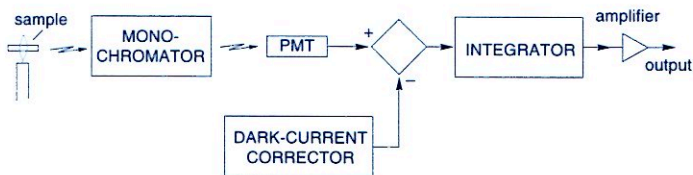
Fig.8.3 Principle of emission spectrometry
