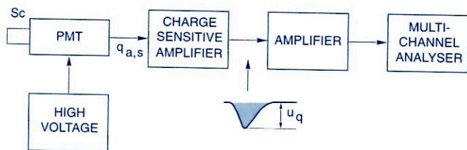
Fig.6.19 Energy spectrometer using a multichannel pulse-height analyser
