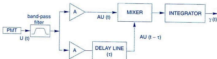
Fig.5.38 Autocorrelation detector
