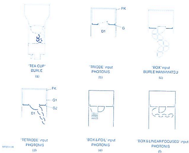
Fig.7.2 Examples of \gamma -camera tube input systems
