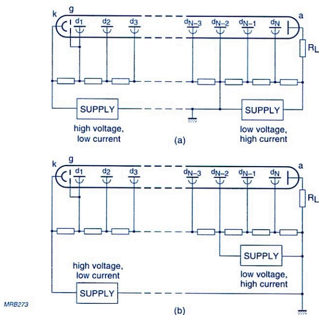
Fig.5.9 Dual voltage supplies: (a) series, (b) parallel
