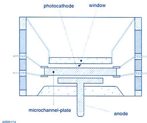
Fig.1.14 Section through a microchannel-plate photomultiplier
