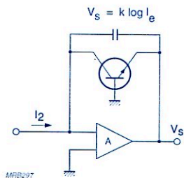
Fig.5.35 Logarithmic amplifier
