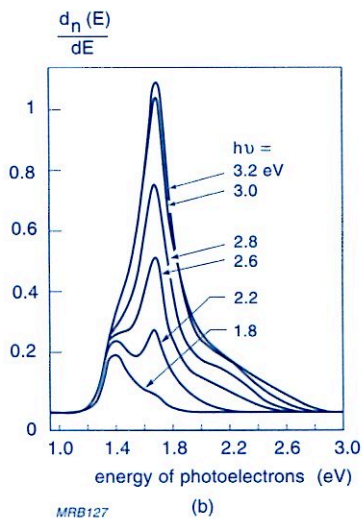
Fig.A1.9 Photoelectron energy distribution (in electrons per photon per eV) from a layer of GaAs(Cs) for incident-photon energies (a) from 1.4 eV to 2.2 eV, and (b) from 1.8 eV to 3.2 eV
