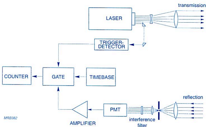
Fig.8.8 Principle of laser telemetry
