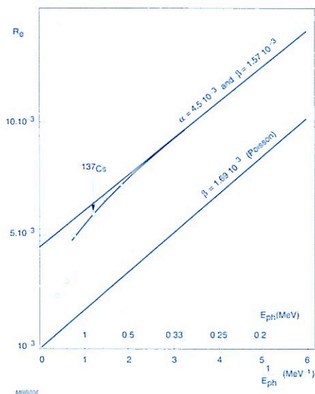
Fig.3.9 Energy resolution as a function of the X or \gamma photon energy E absorbed in the scintillator
