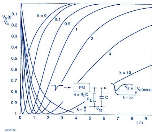
Fig. 6.11 Relative pulse amplitude shapes for an anode load R_L C with k = \theta/\tau as parameter and the amplitudes normalized to 1
