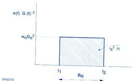
Fig.A3.1 Definition of noise pass-band B_N .
