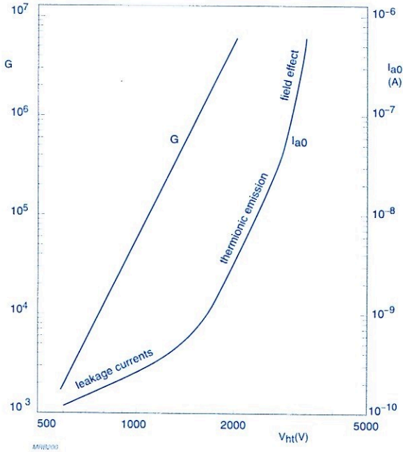
Fig.3.2 Major causes of dark current versus supply voltage
