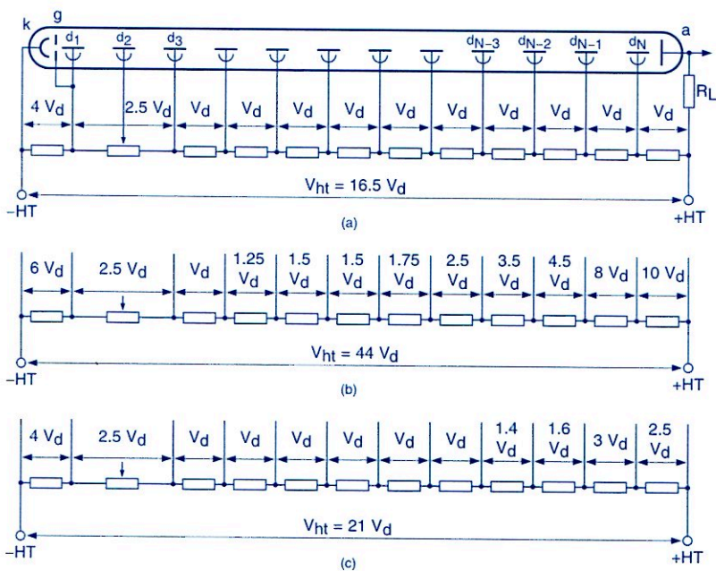
Fig.5.7 Voltage dividers: (a) type A equal step, (b) type B progressive, (c) type C intermediate
