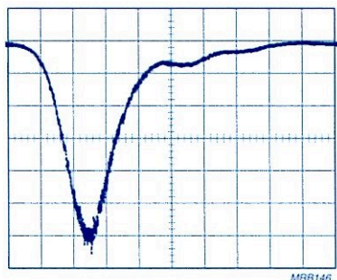
Fig.2.5 Anode current pulse response of a fast-response photomultiplier: vertical scale 20 mA/div., horizontal scale 2 ns/div
