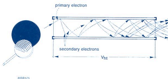
Fig.1.15 Electron multiplication in a microchannel
