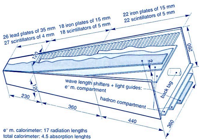
Fig.7.15 Calorimeter tower based on the wavelength shifter principle (courtesy of CERN, experiment UA 2)
