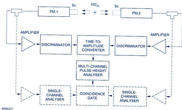
Fig.6.26 Basic setup for time spectrometry
