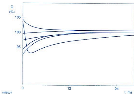
Fig.4.21 Examples of initial low-current drift
