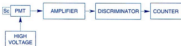
Fig.6.15 Block diagram of a scintillator pulse counter
