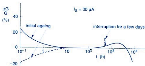
Fig.4.20 Relative gain variation of a photomultiplier operating at high average current
