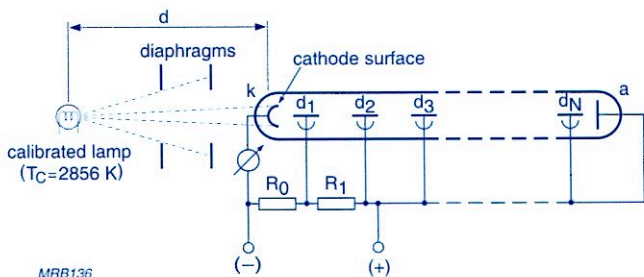
Fig.2.11 Set-up for measuring cathode sensitivity
