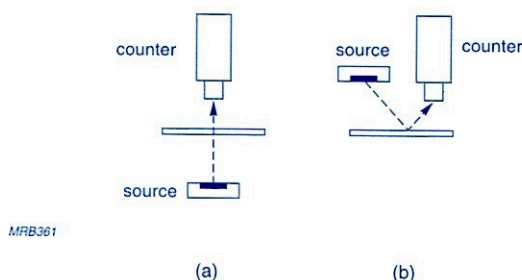
Fig.7.12 Principle of thickness measurement (a) by transmission, (b) by reflection
