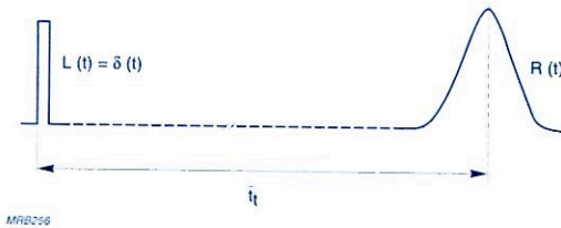
Fig.A4.5 Pulse transit-time probability distribution
