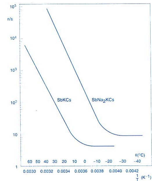
Fig.3.1 Number of dark pulses per second as a function of temperature, for SbKCs and SbNa 2 KCs photocathodes
