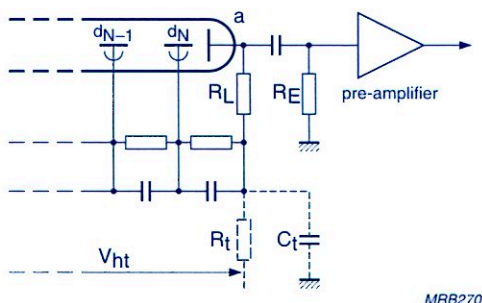
Fig.5.6 Network for decoupling the high-voltage switch-on transient from the amplifier input
