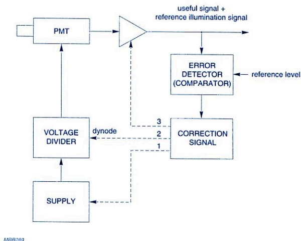
Fig.5.27 Correction of anode-sensitivity drift by varying the gain. The signal due to a reference illumination of the cathode is compared with a fixed reference level to derive an error signal. The gain can be altered by any one of the three routes shown
