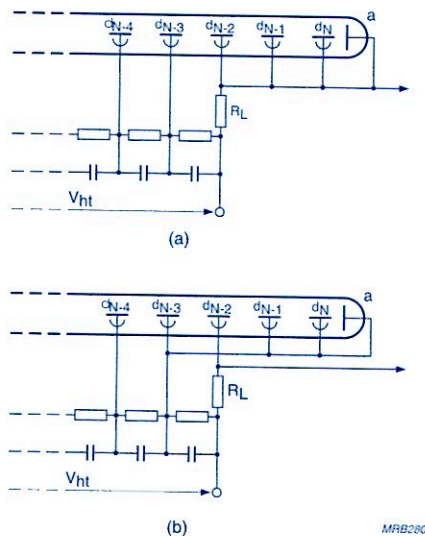
Fig.5.16 Reducing the number of active stages
