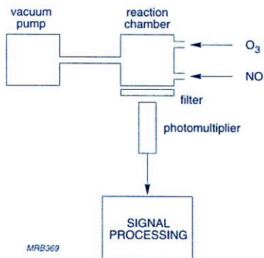
Fig.8.2 Measurement of chemiluminescence
