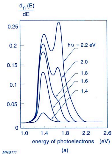
Fig.A1.9 Photoelectron energy distribution (in electrons per photon per eV) from a layer of GaAs(Cs) for incident-photon energies (a) from 1.4 eV to 2.2 eV, and (b) from 1.8 eV to 3.2 eV
