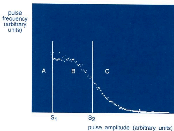
Fig.5.41 Pulse-amplitude spectrum of photomultiplier operating under single-electron conditions, showing lower and upper thresholds for photon counting (defining counting window B)
