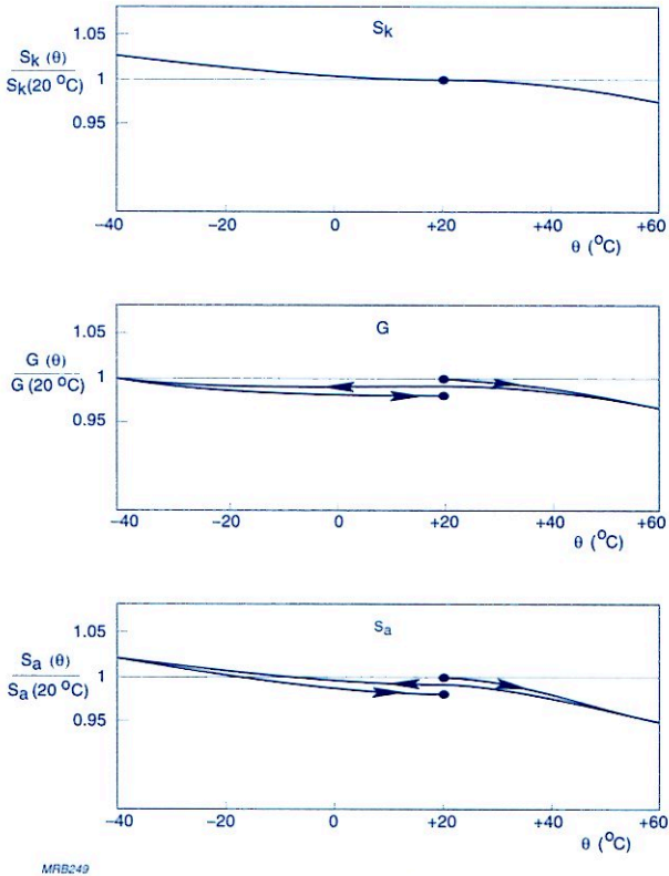
Fig.4.34 Temperature variation of cathode and anode sensitivity and gain of a tube with a bi-alkali cathode at a wavelength of 405 nm, showing hysteresis.
