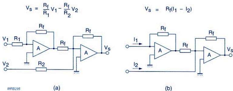
Fig.5.33 (a) Voltage subtractor, (b) current subtractor
