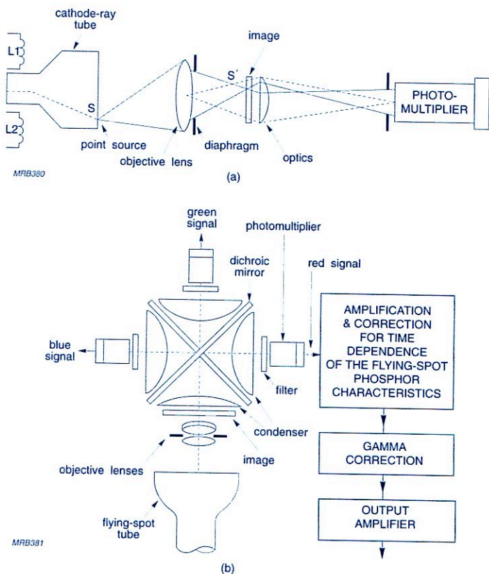
Fig.8.7 Conversion of photo-transparencies into a video image using a flying-spot scanner and photomultiplier tubes (a) monochrome system, (b) three-colour system
