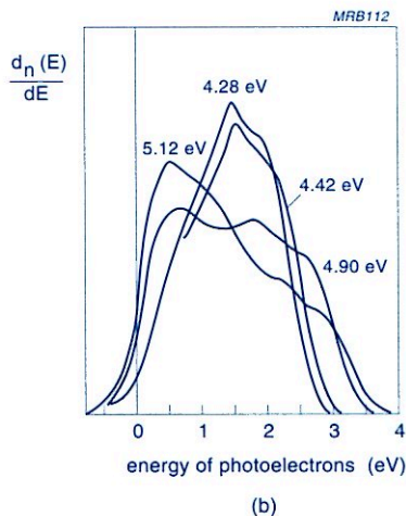
Fig.A1.8 Relative distribution of photoelectron energies, E_{ph} , from a layer of SbKCs at 290 K, for incident photon energies (a) from 2.15 eV to 3.06 eV, and (b) from 4.28 eV to 5.12 eV
