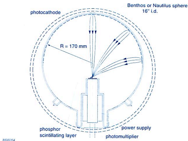
Fig.1.18 Smart photomultiplier combination in a glass pressure sphere for deep underwater muon and neutrino detectors (DUMAND)
