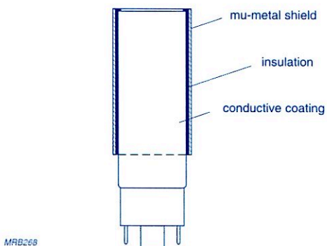
Fig.5.4 Magnetic shielding, insulation, and conductive coating
