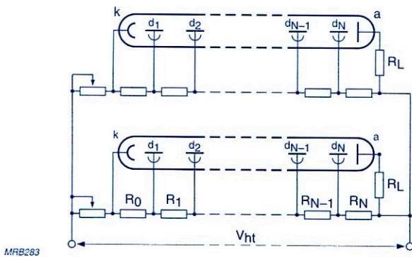
Fig.5.21 High-voltage supply to photomultipliers in parallel
