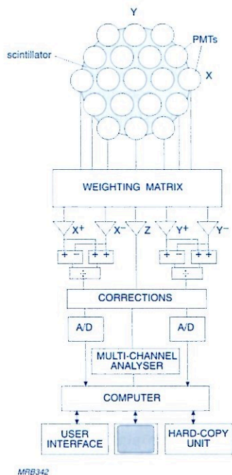
Fig.7.1 Operating principle of a \gamma -camera
