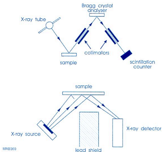
Fig.7.11 Schematic diagram of two X-ray spectrometers (a) dispersive, (b) non-dispersive
