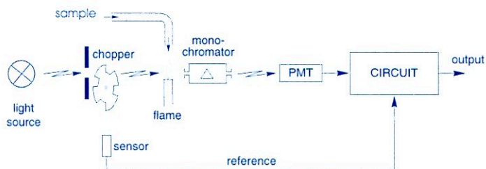
Fig.8.5 Principle of absorption spectrometry
