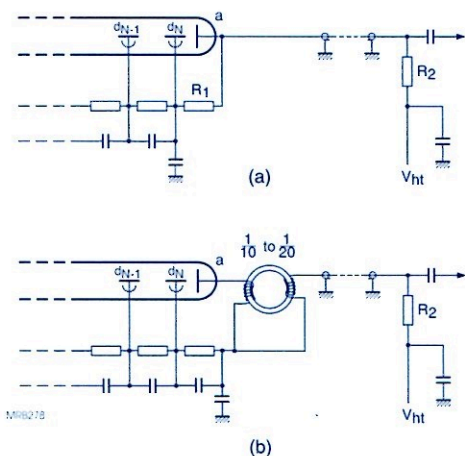
Fig.5.14 Voltage supply via the output cable
