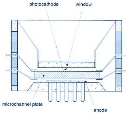
Fig.1.17 Microchannel-plate photomultiplier with mosaic anode
