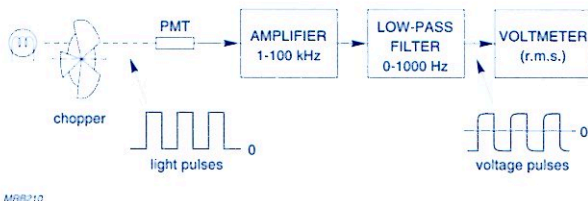
Fig.3.13 Set-up for measuring noise equivalent power
