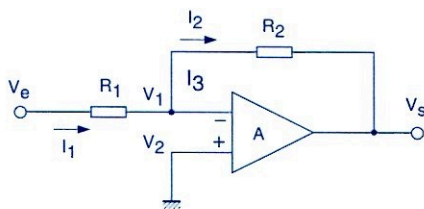
Fig.5.30 Voltage amplifier (inverting)
