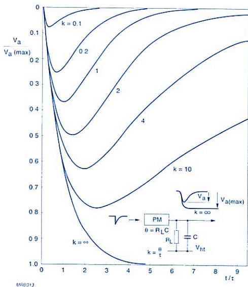
Fig. 6.10 Relative pulse amplitude shapes for an anode load R_L C with k = \theta/t as parameter
