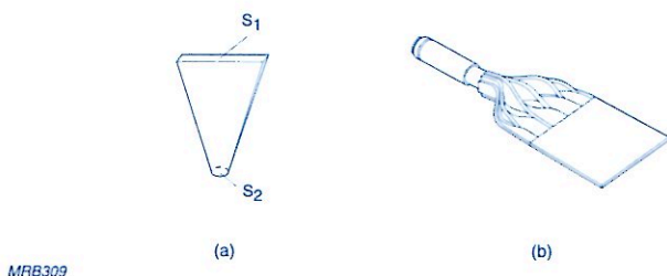
Fig.6.6 The fishtail (a) and strip-light (b) are two examples of light guides designed to adapt specially shaped scintillators to circular cathode windows
