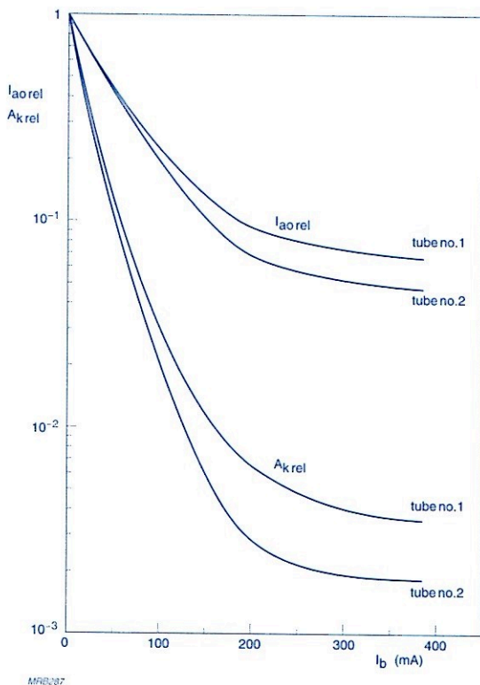
Fig.5.25 Relative dark-current ( I_{a0} ) and cathode-area ( A_k ) reduction as functions of solenoid current I_b in two tubes with 32 mm diameter S1 cathodes, using the method of Fig.5.24.
