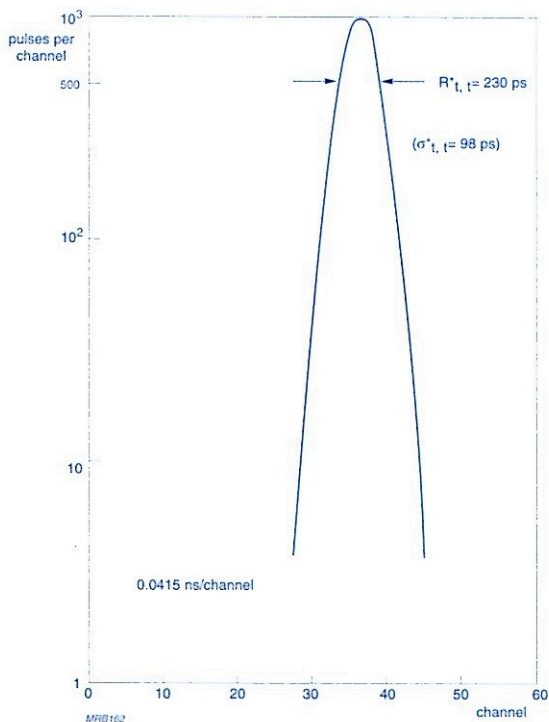
Fig.6.27 Coincidence time resolution distribution from two fast scintillation counters for ^{60}\text{Co} coincidence \gamma\text{-}\gamma radiation
