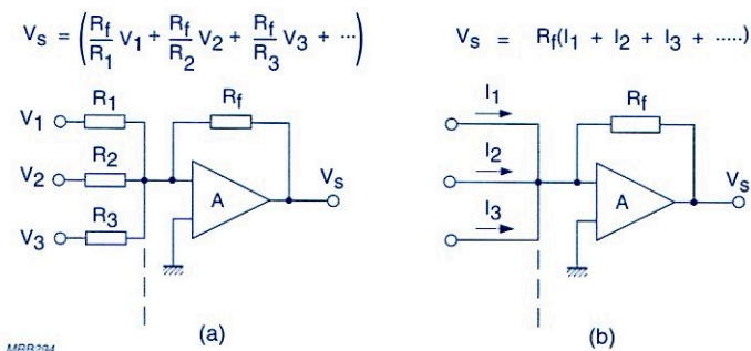
Fig.5.32 (a) Voltage adder, (b) current adder
