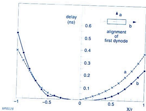
Fig.4.7 Transit-time differences of a fast-response photomultiplier as functions of distance from the cathode centre, measured along perpendicular diameters
