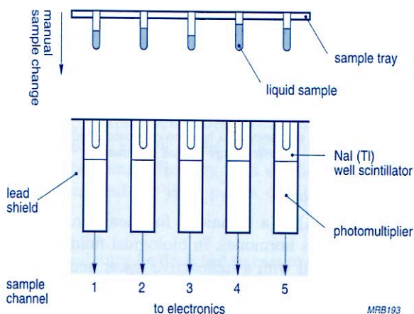
Fig.7.8 RIA counter with 5 channels
