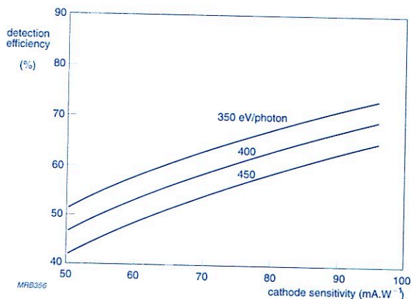
Fig.7.7 Detection efficiency as a function of photocathode sensitivity for ^3\text{H} , with energy loss as parameter
