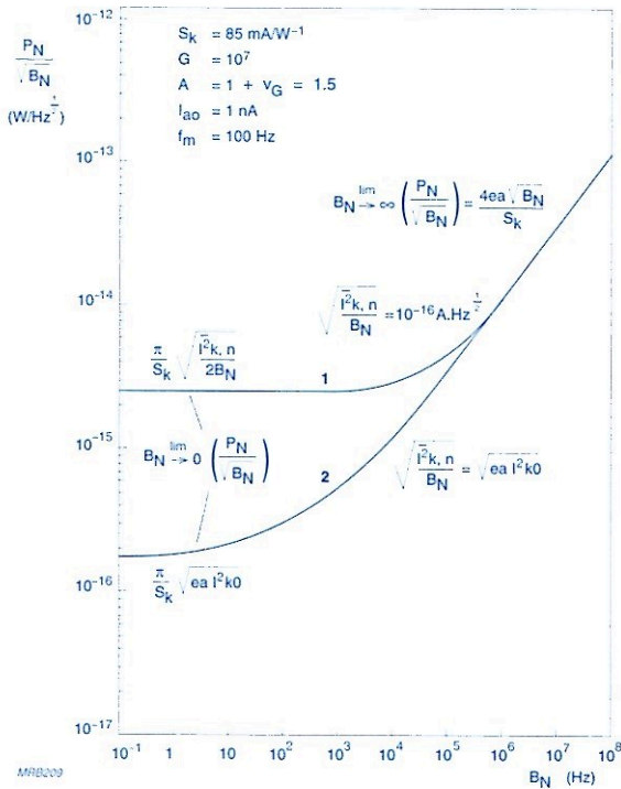
Fig.3.12 Noise equivalent power (flux as a function of the measuring circuit passband, for two value of additional noise: 1) 10^{-16} A/Hz 1/2 , 2) 7 \times 10^{-18} A/Hz 1/2
