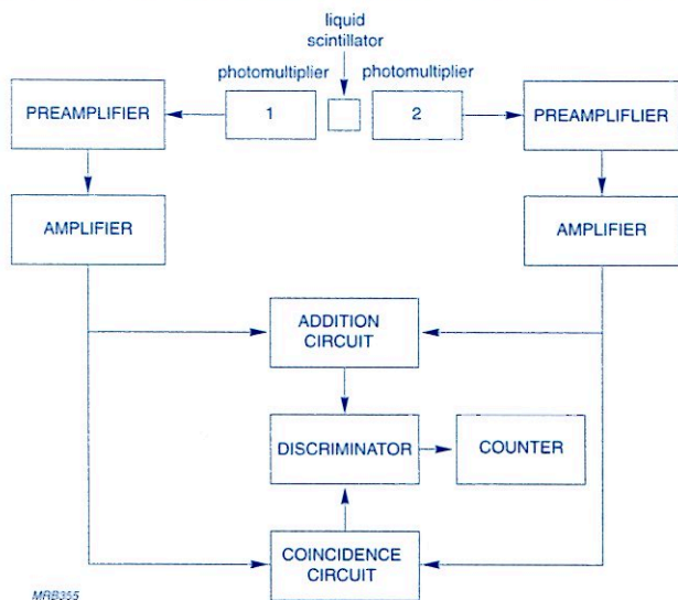
Fig.7.6 Schematic diagram of a liquid scintillation counter
