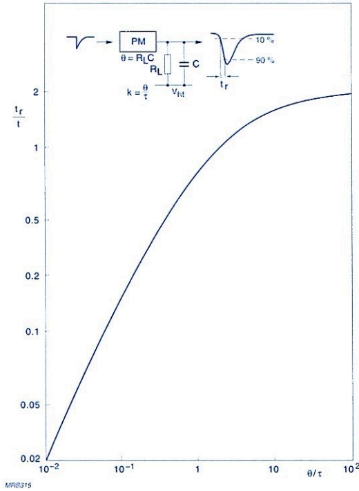
Fig.6.12 Variation of pulse rise time with \theta/\tau
