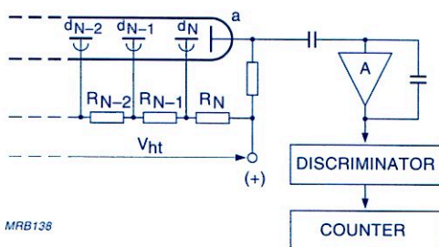
Fig.2.13 Dark-pulse-rate measurement
