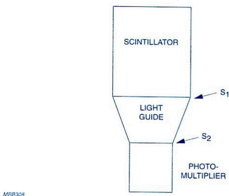
Fig.6.5 Truncated cone light guide
