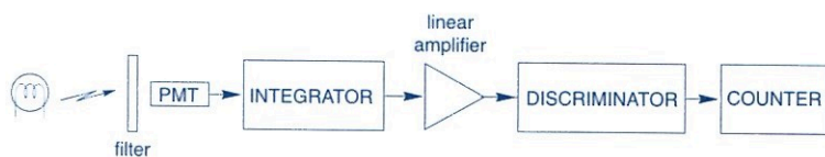
Fig.5.40 Photon-counting detector
