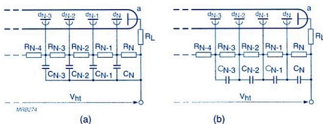
Fig.5.10 Dynode decoupling: (a) parallel, (b) series.
