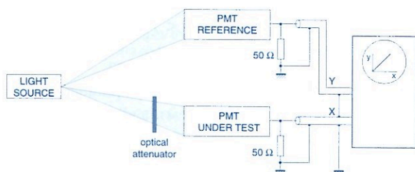
Fig.4.16 Set-up for the XY-method of measuring linearity
