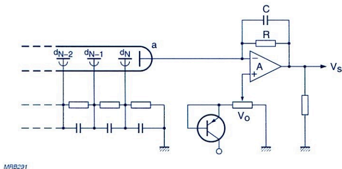
Fig.5.29 Circuit for compensating temperature-dependent dark-current drift
