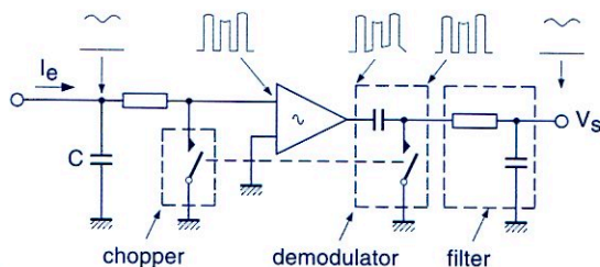
Fig.5.36 Chopper-stabilized amplifier
