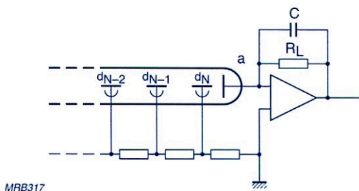
Fig.6.14 Circuit for a photomultiplier in continuous mode
