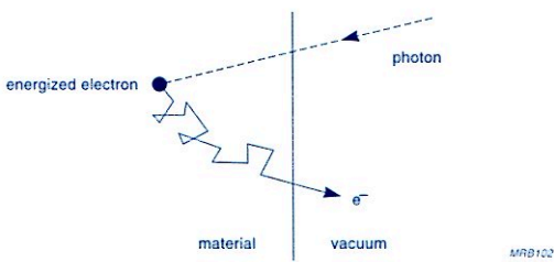
Fig.A1.1 Photoemission
