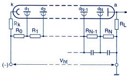
Fig.5.2 Negative-polarity voltage supply
