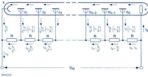
Fig.4.11 Current distribution in an iterative voltage divider
