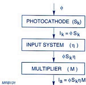
Fig.2.3 Photomultiplier sensitivity characteristics
