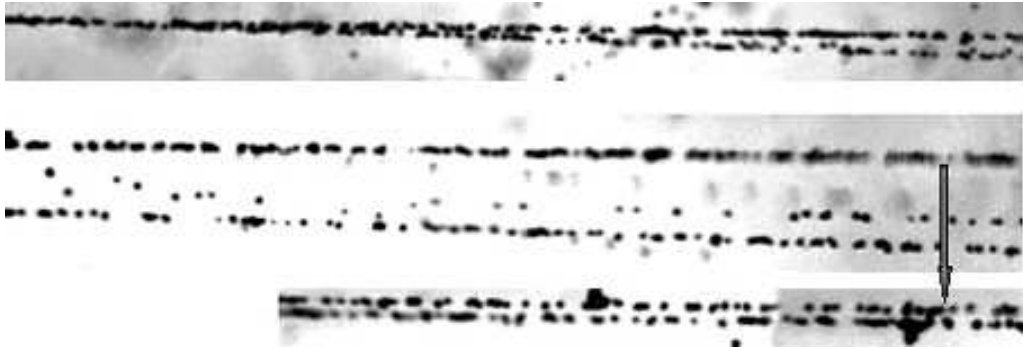
Fig. 7. Event of dissociation of a 4.5A GeV/ c ^{14}\text{N} nucleus in peripheral interaction into three He and one H fragments. Upper photo: interaction vertex with production of a narrow fragment jet. Middle photo: shifting from vertex allows one to identify single H and He relativistic fragments accompanied by a very close track pair (top). Lower photo: further shifting allows one to resolve the central pair on the previous photo as a relativistic ^8\text{Be} production.
