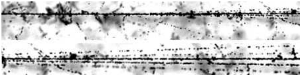
Fig. 11. Event of dissociation of 4.5A GeV/ c ^{24}\text{Mg} nucleus in peripheral interaction into charged topology 1+1+7+2+1 (from top to bottom). Upper photo: interaction vertex with production of narrow fragment jet accompanied with a relativistic meson like track. Lower photo: shifting from vertex allows one to resolve five fragments.
