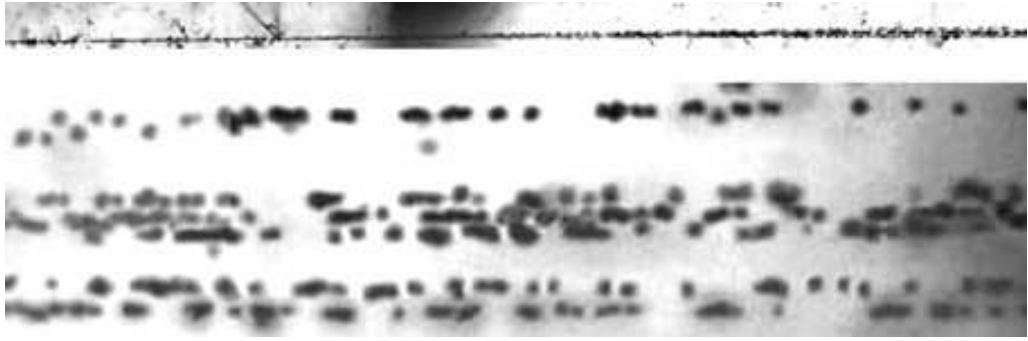
Fig. 14. Event of dissociation of a 4.5A GeV/ c ^{24}\text{Mg} nucleus in peripheral interaction into six He fragments. Upper photo: interaction vertex with production of a narrow fragment jet accompanied with a couple of target slow fragments. Lower photo: further shifting allows one to resolve (from top to bottom) separate He fragment, very narrow He fragment triple (most probably, decay of excited ^{12}\text{C} nucleus), and a very narrow He pair ( ^8\text{Be} production).
