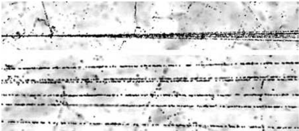
Fig. 15. Event of dissociation of a 4.5A GeV/ c ^{24}\text{Mg} nucleus in peripheral interaction into five \alpha particles and single ^3\text{He} fragments. Upper photo: interaction vertex with production of narrow fragment jet accompanied with a target recoil. Lower photo: further shifting allows one to resolve (from top to bottom) a six He fragment system containing a very narrow \alpha particle pair ( ^8\text{Be} production).
