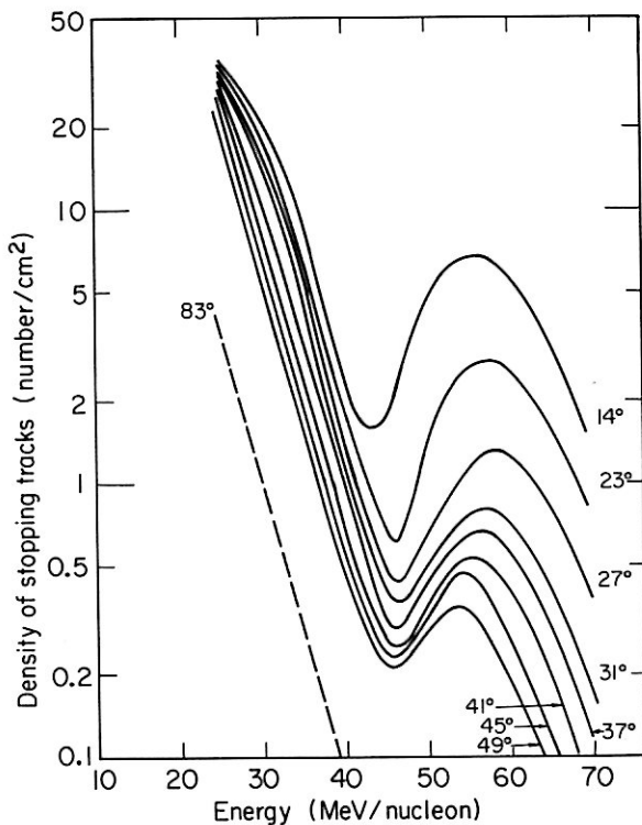
9. Energy distribution of ^{12}\text{C} fragments produced at various angles in the reaction ^{12}\text{C} + ^{198}\text{Au} \rightarrow ^{12}\text{C} + \text{anything} for 2.1 GeV/nucleon ^{12}\text{C} projectiles. Experiment of Crawford et al. (see section III-C).
