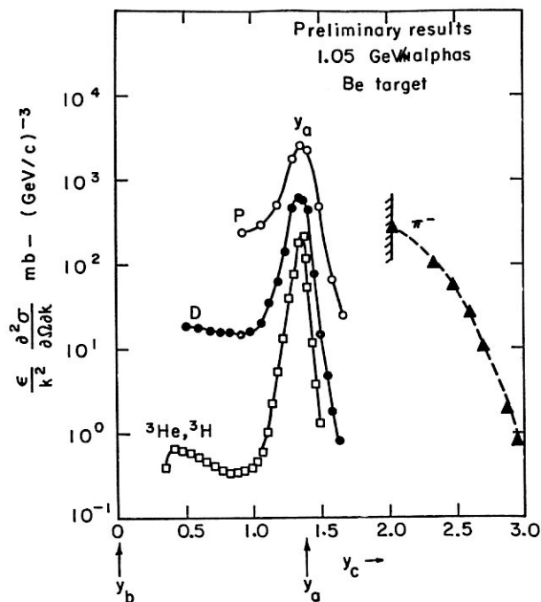
15. Invariant cross section, E/k^2 d^2\sigma/d\Omega dk as a function of fragment rapidity for proton, deuteron, ^3\text{H} and ^3\text{He} fragments produced by 1.05 GeV/nucleon alpha particle projectiles on Be. Data of Papp et al. (see section III-D).
