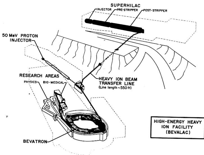
1. Schematic view of Bevalac showing SuperHILAC injector, transfer line, and Bevatron.
