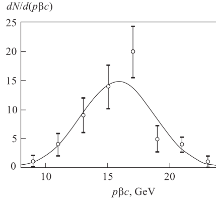
Fig. 4. Reconstructed distribution over p\beta c for beam double charged tracks
