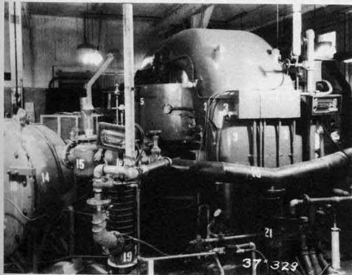
Fig. 2. The 37-inch synchrocyclotron. The cylindrical tank at the left houses the rotating condenser.
