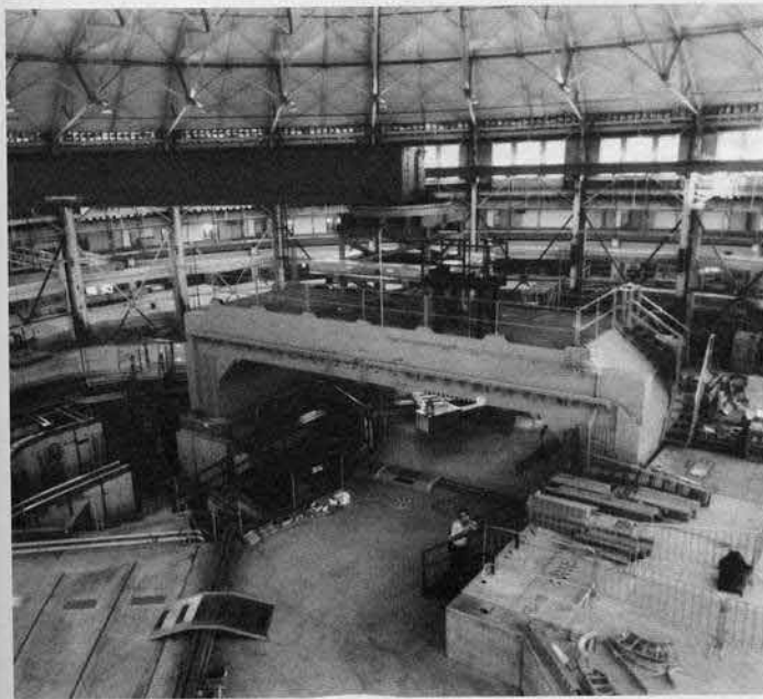
Fig. 5. The Advanced Light Source, with the yoke of the 184-inch cyclotron magnet in the center. 1994.
