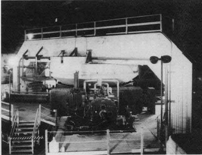
Fig. 4. The 184-inch Synchrotron as completed in 1946.
