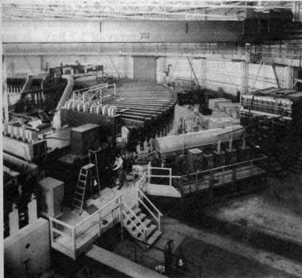
Fig. 11. The Bevatron as completed, without shielding, injector linac and Cockcroft-Walton pre-injector at the right.
