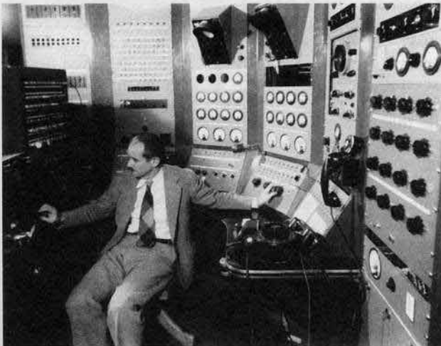
Fig. 8. With one hand on the injection timing control and the other on an oscilloscope, McMillan operates the Synchrotron.
