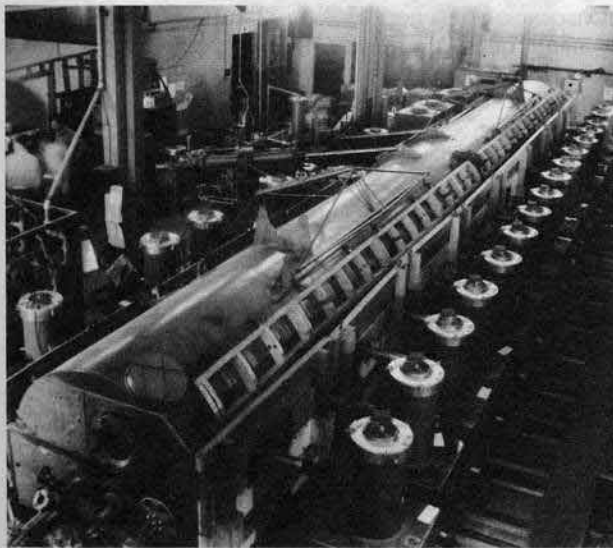
Fig. 9. The Alvarez linear Accelerator.
