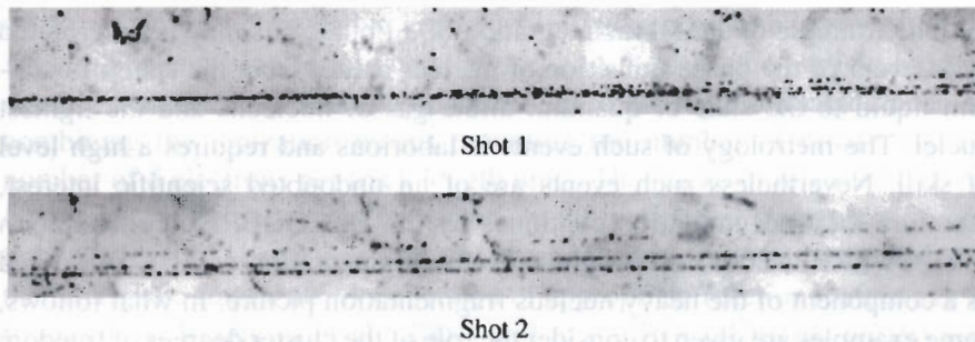
Figure 2. Subsequently reconstructed photo of dissociation of a 1 A GeV ^{10}\text{B} nucleus into 1 doubly and 2 singly charged fragments without production of target nucleus fragments and mesons ("white"star): interaction vertex (Shot 1); apparent tracks of 1 H and 2 He nuclei (from top to bottom, Shot 2).
