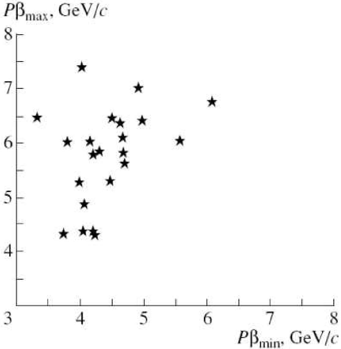
FIG. 3: The distribution of the “white” stars from a {}^7\text{Be} nucleus of the energy of 1.23 GeV per nucleon with a decay to two He fragments with respect to minimum and maximum momenta.
