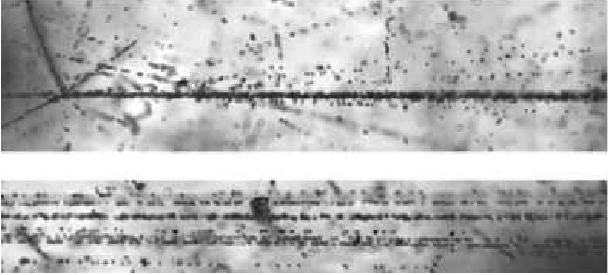
FIG. 1: Event of the fragmentation of a ^{28}\text{Si} nucleus of the energy of 3.65 GeV per nucleon in a peripheral interaction on an emulsion nucleus. On the upper photograph one can see the interaction vertex and the jet of fragments in a narrow angular cone along with four accompanying singly charged particles in a wide cone and three fragments of the target-nucleus. Moving toward the fragment jet direction (upper photograph) it is possible to distinguish 3 fragments of hydrogen and 5 fragments of helium. An intensive track on the upper photograph (the third one from above) is identified as a very narrow pair of Z=2 fragments corresponding to the ^8\text{Be} decay. A 3-dimensional image of the event was reconstructed as a plane projection by means of an automated microscope (Lebedev Institute of Physics, Moscow) of the PAVIKOM complex.
