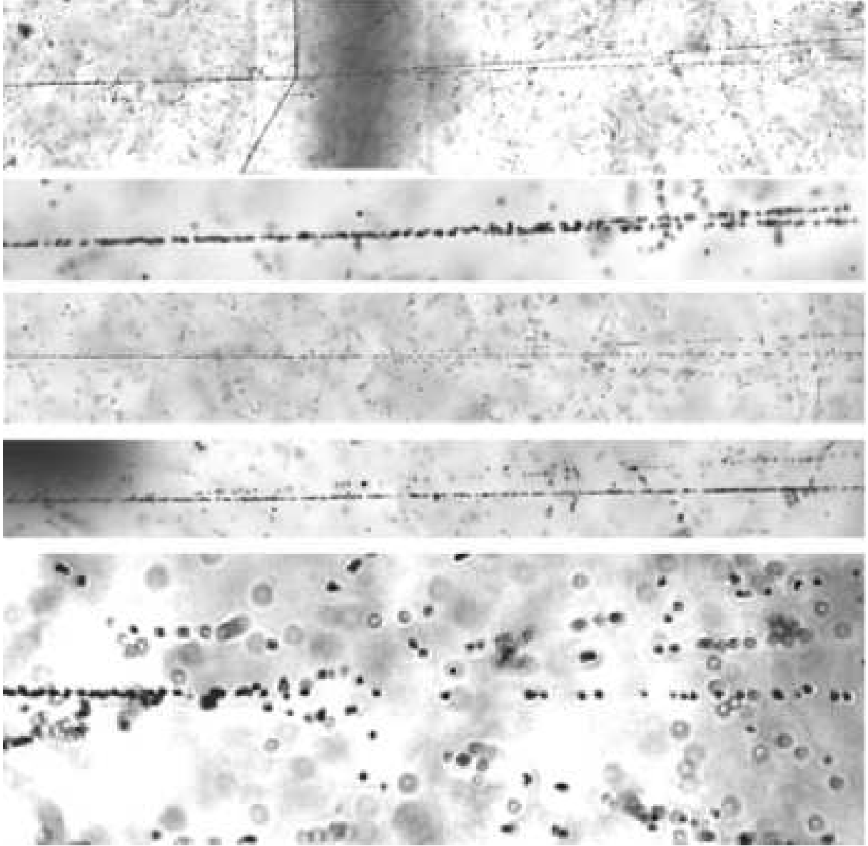
FIG. 2: Examples of the events from the peripheral {}^7\text{Be} dissociation in emulsion. The upper photograph is a splitting to two He fragments with production of two target-nucleus fragments. Below there are “white” stars with splitting to two He, one He and two H, one Li and one H and four H fragments.
